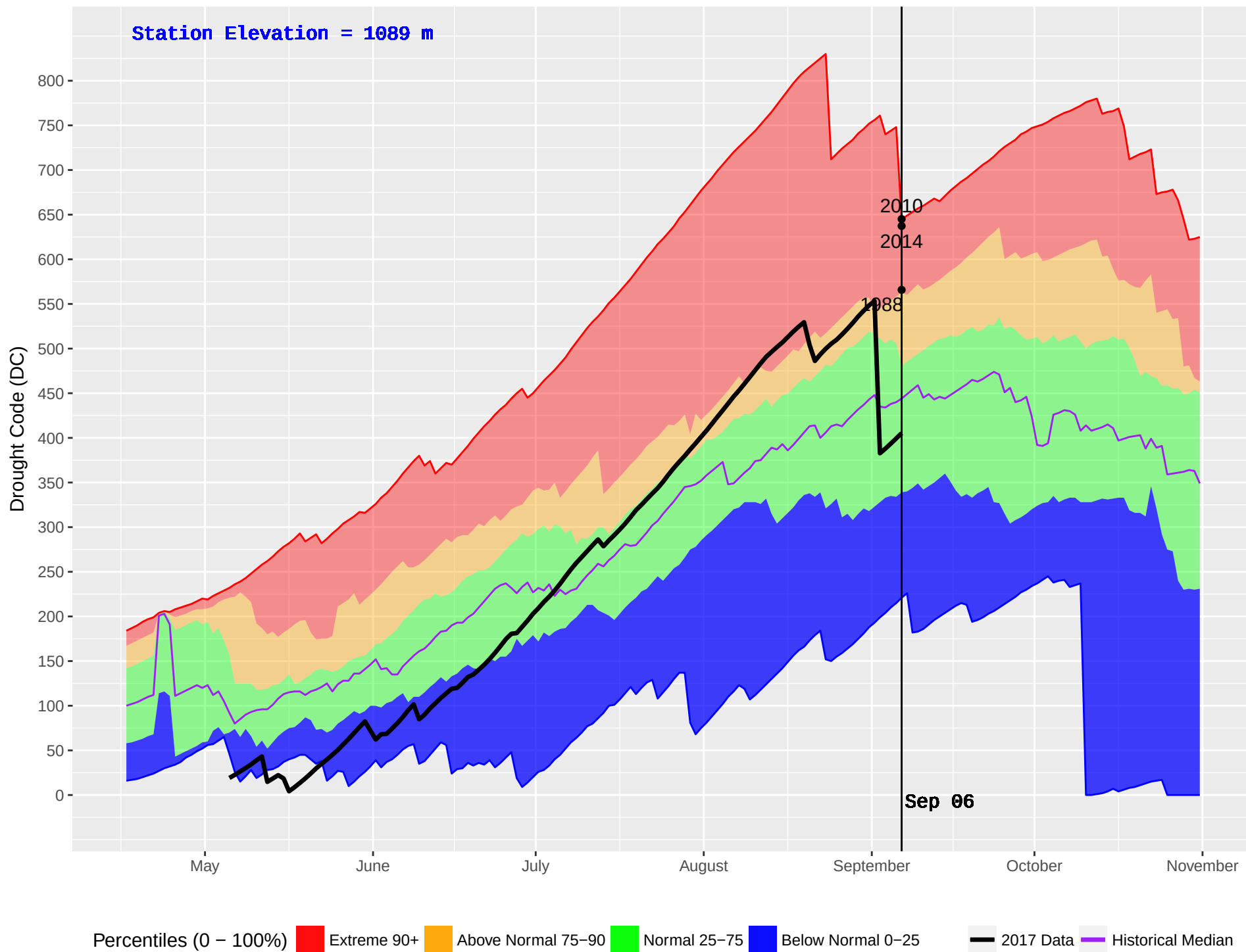
EAST OOTSA (170) : Historical (1986–2016) and Current (2017) Noon Drought Code (DC)
