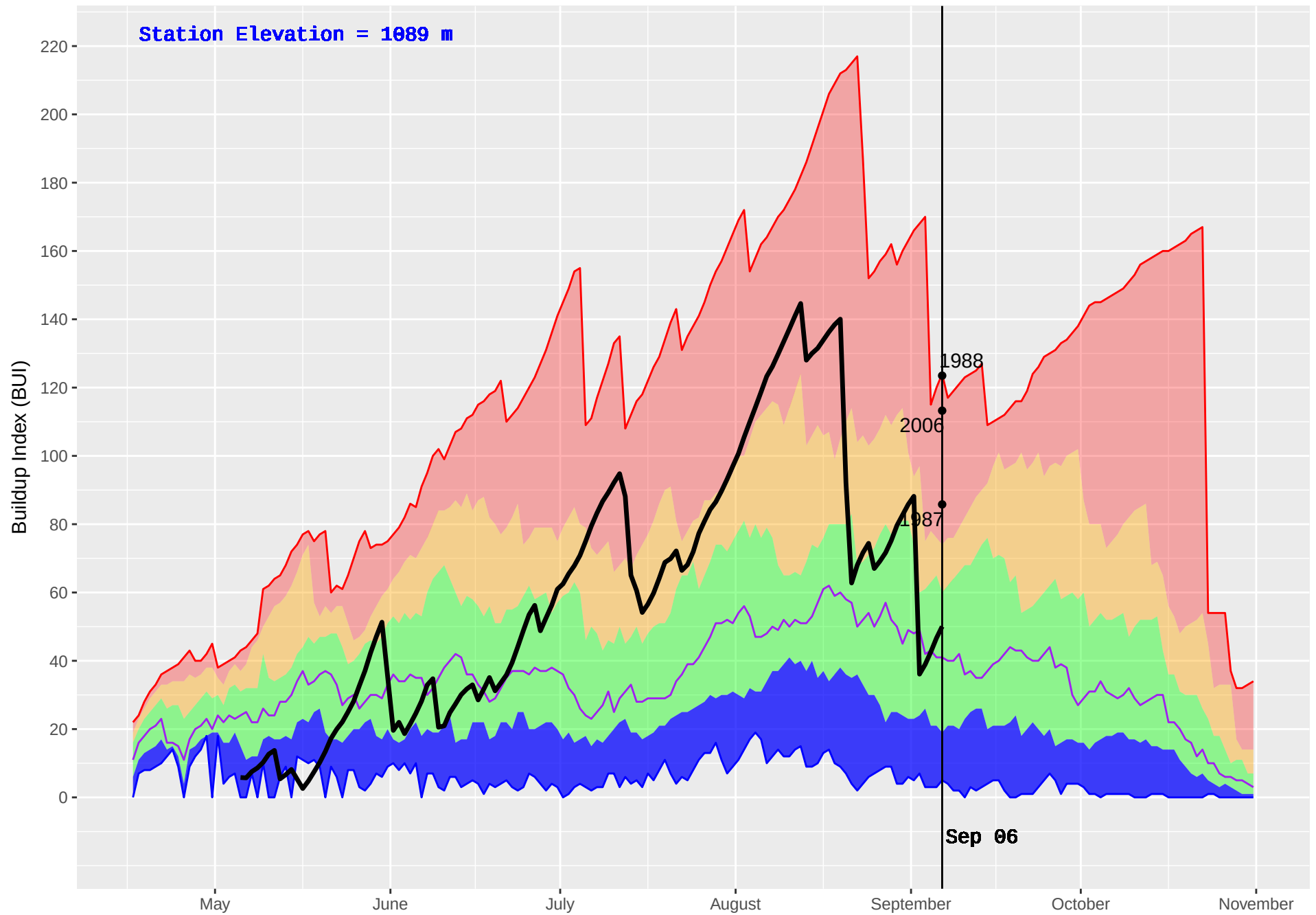
EAST OOTSA (170) : Historical (1986–2016) and Current (2017) Noon Buildup Index (BUI)
