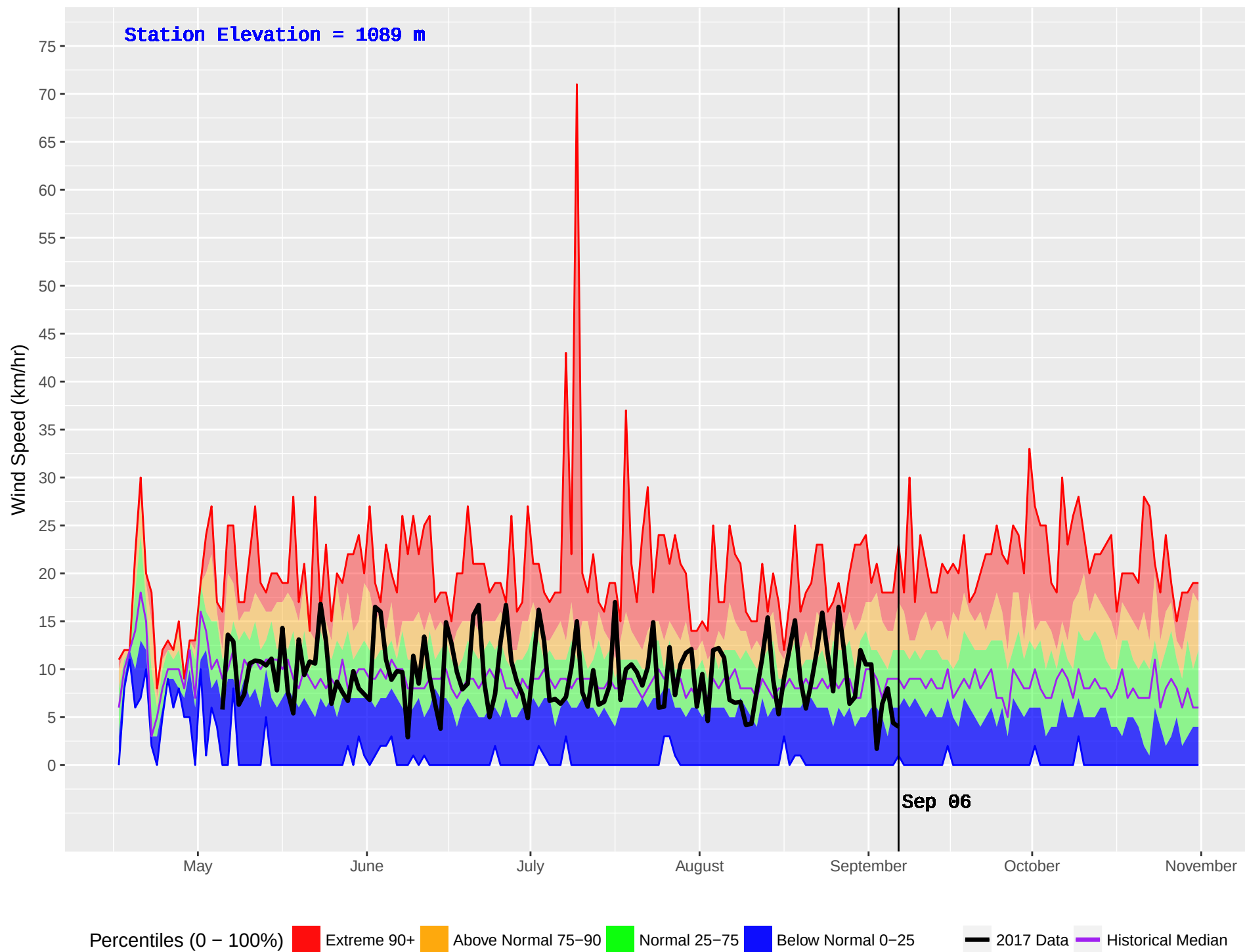
EAST OOTSA (170) : Historical (1986–2016) and Current (2017) Noon Wind Speed
