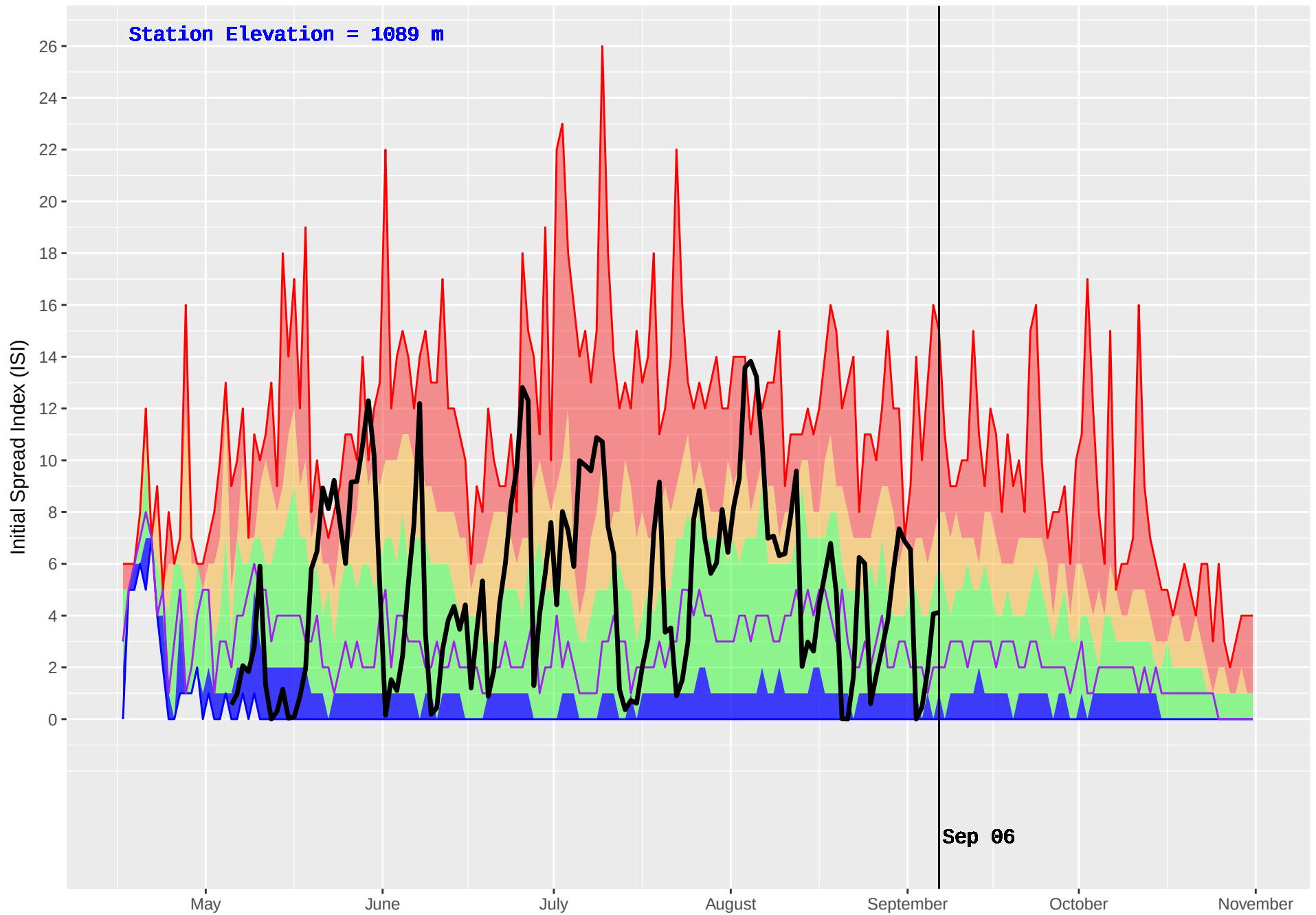
EAST OOTSA (170) : Historical (1986–2016) and Current (2017) Noon Initial Spread Index (ISI)
