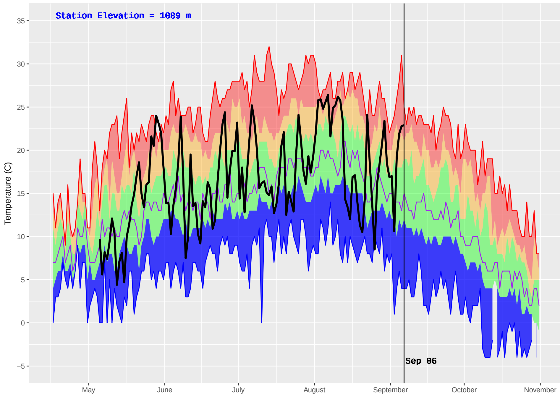
EAST OOTSA (170) : Historical (1986–2016) and Current (2017) Noon Temperature
