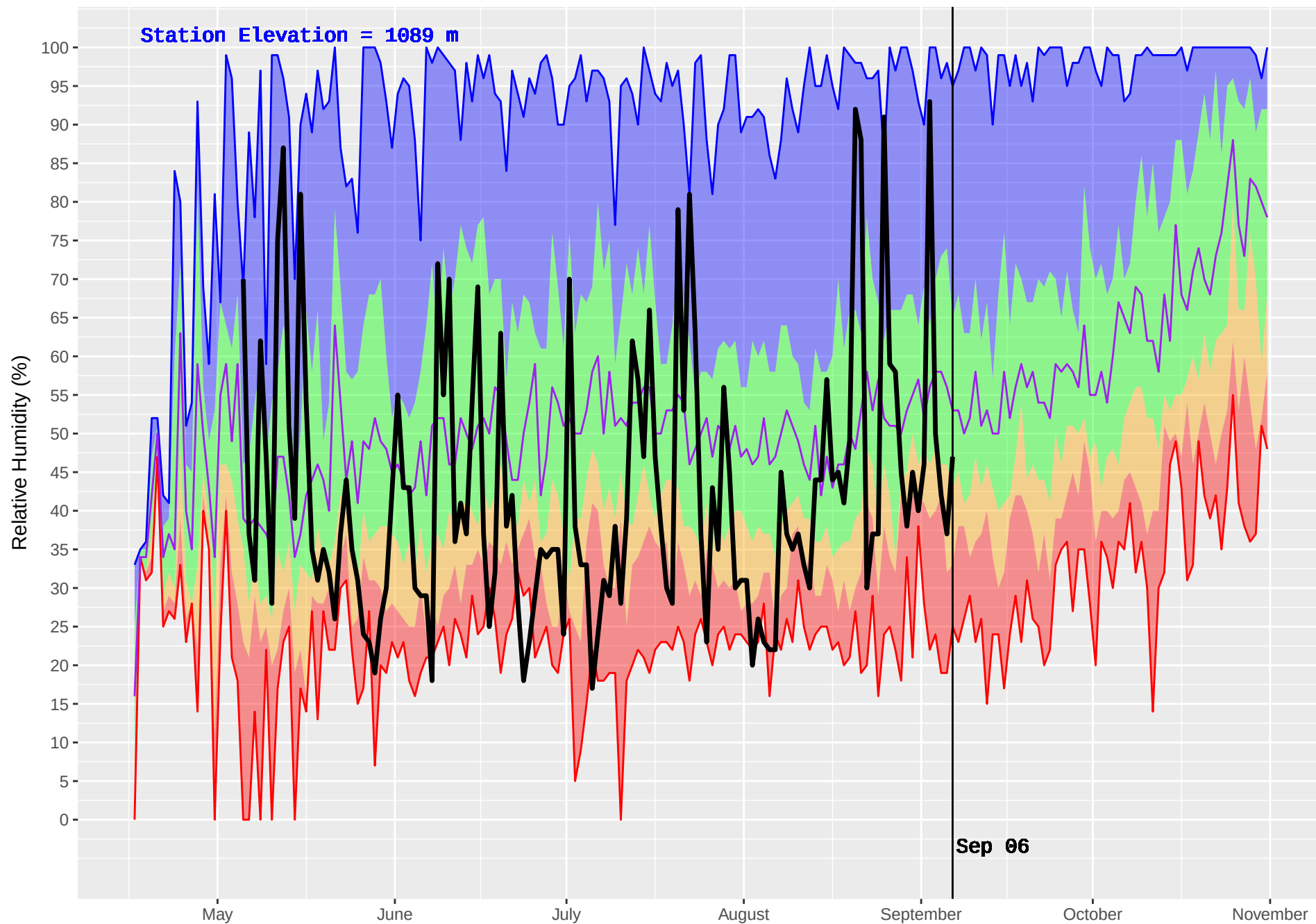
EAST OOTSA (170) : Historical (1986–2016) and Current (2017) Noon Relative Humidity
